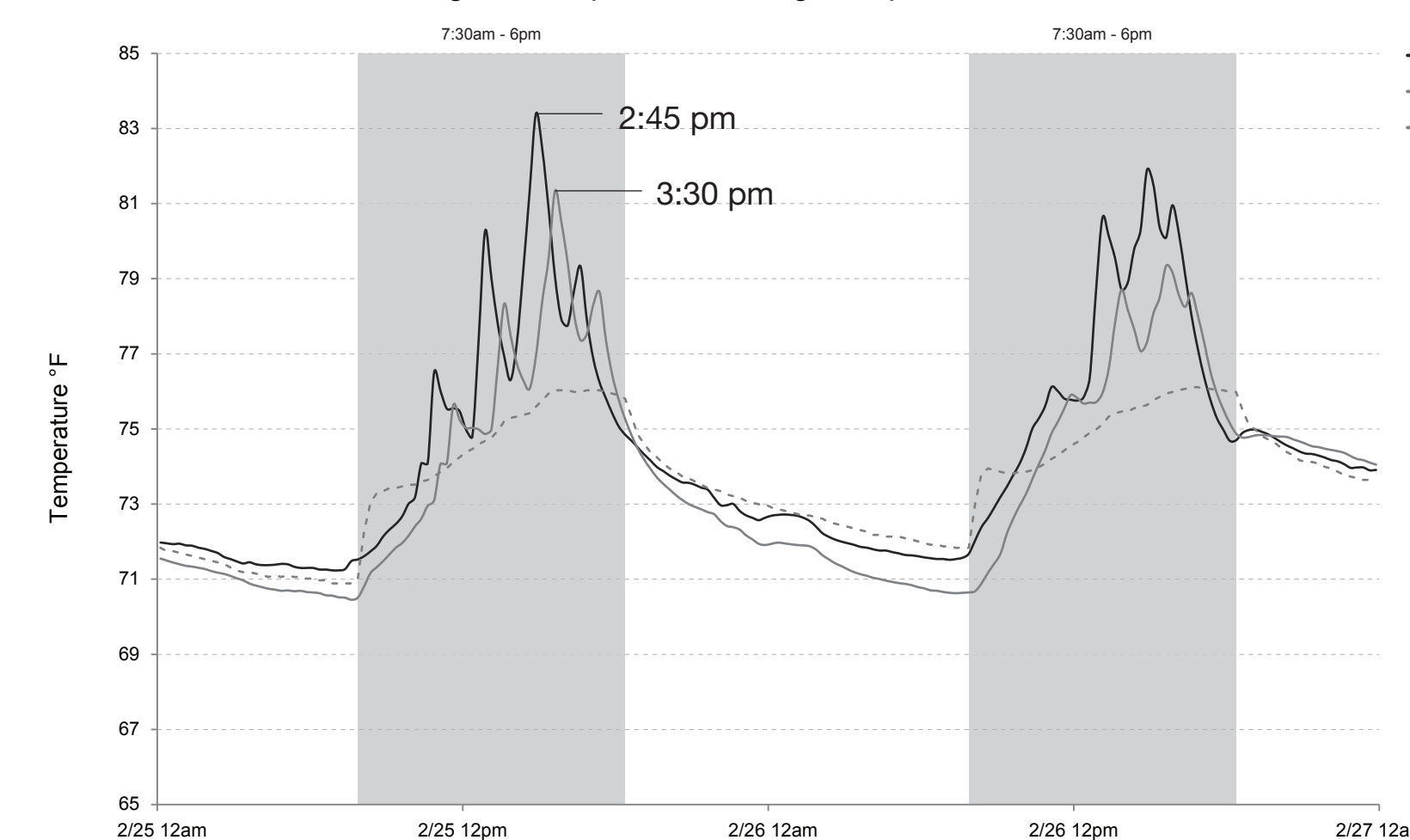
Average air temperature ceiling/occupied/ventilation zone
